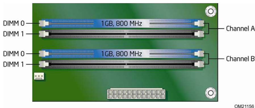
Figure 14. Dual Channel Memory Configuration with Two DIMMs
